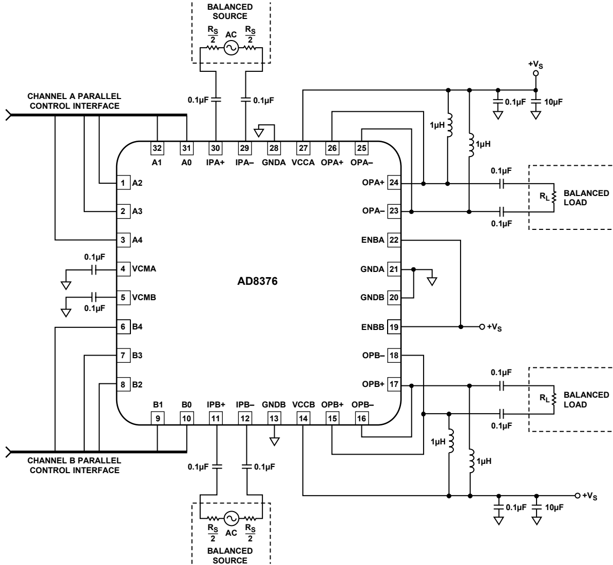
Figure 36. Basic Connections
