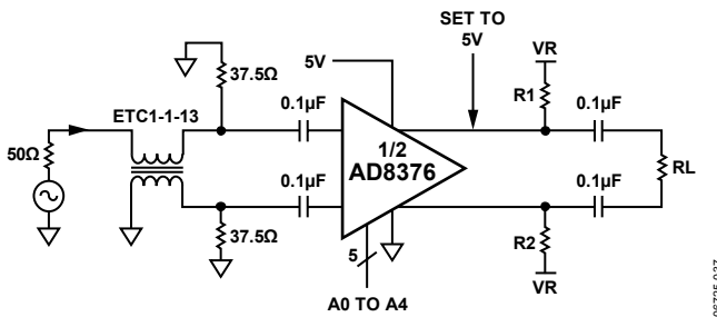
Figure 37. Single-Ended Broadband Operation with Resistive Pull-Ups
