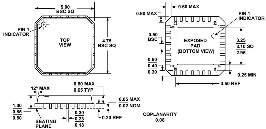
Figure 52. 32-Lead Lead Frame Chip Scale Package [LFCSP_VQ] 5 mm × 5 mm Body, Very Thin Quad (CP-32-2) Dimensions shown in millimeters
