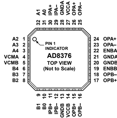
Figure 3. 32-Lead LFCSP
